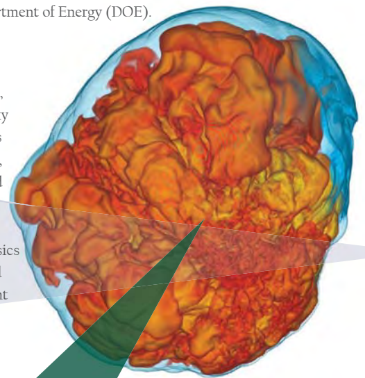
High fidelity computer simulation of a supernova explosion.
